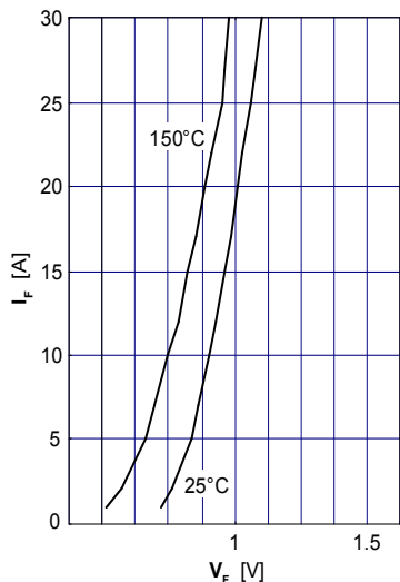
Fig. 1 Forward current versus voltage drop per diode
