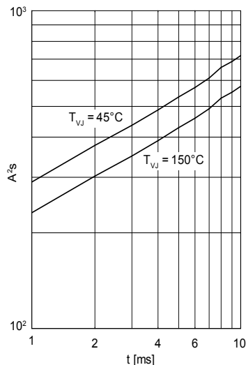
Fig. 3 I^2t versus time (1-10 ms) per diode or thyristor
